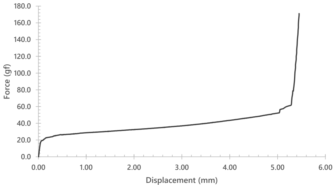
Niz EC Linear UHMWPE 25g (Upstroke)
